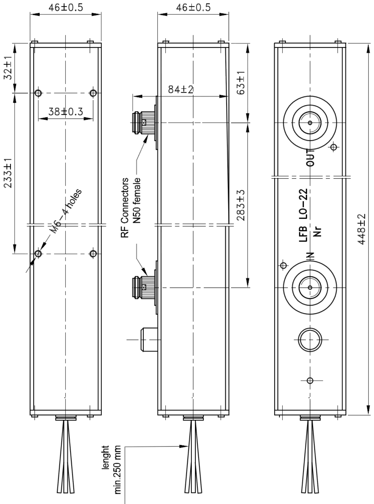
Fig. 2. Dimensions of tube LO-22
