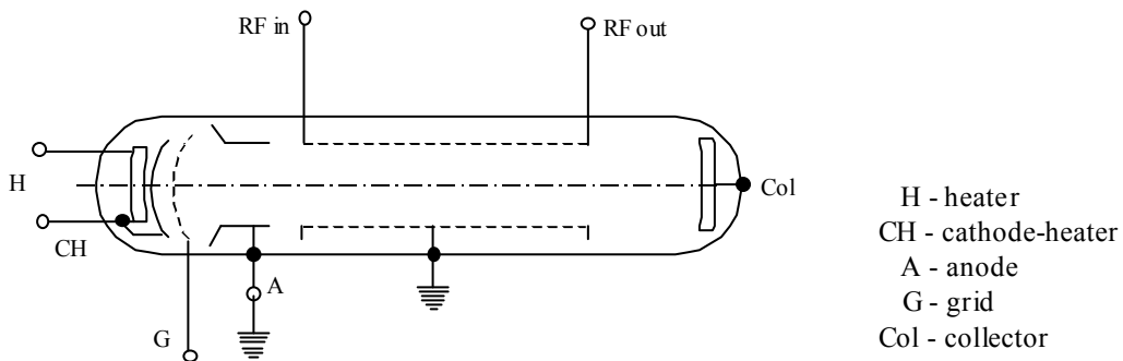
Fig. 1. Scheme connections of electrodes tube LO-22
